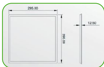
Diagram of 18W 300x300 LED Panel
