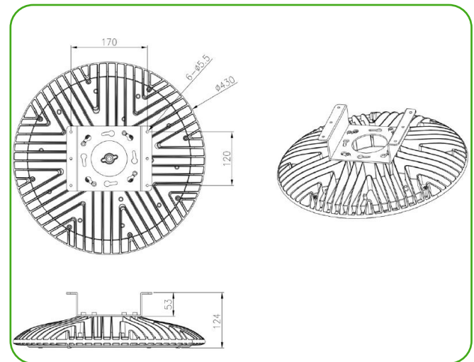
Diagram of Discus Zero (150W, 200W)
