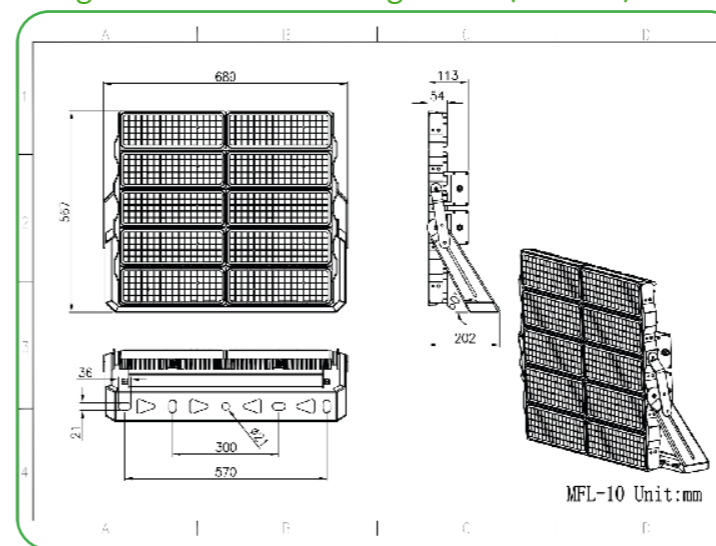
Diagram of Discus Floodlight Plus (1000W) - Other sizes available
