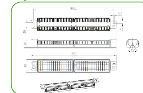
Diagram of Javelin Zero (100W, 150W)
