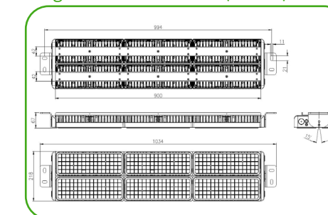
Diagram of Javelin Zero (400W)
