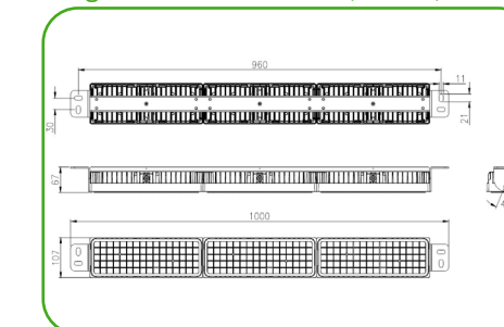
Diagram of Javelin Zero (200W)
